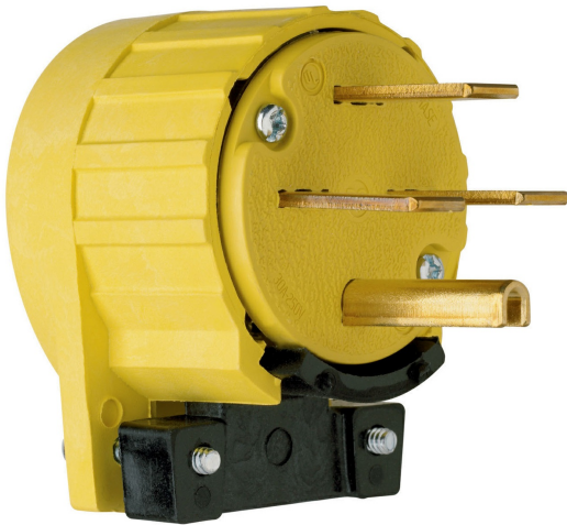
Plug 30A 3-Phase 250V Angle
