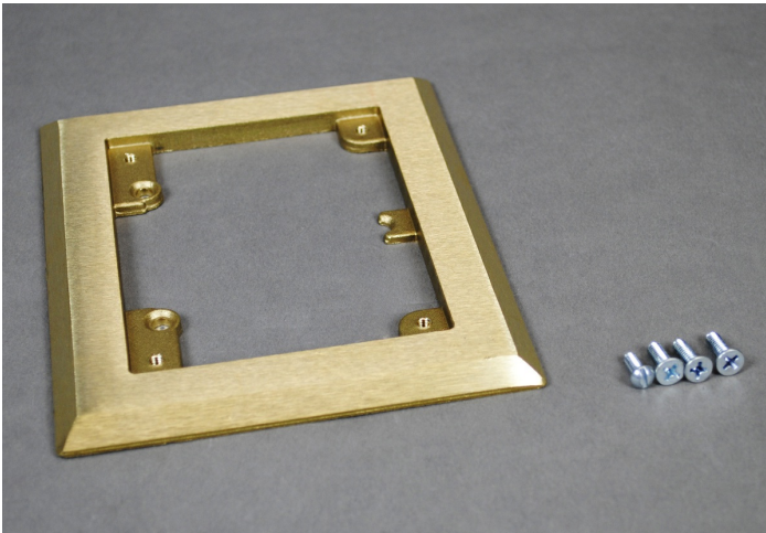
Flush brass carpet flange only with mounting screws.
